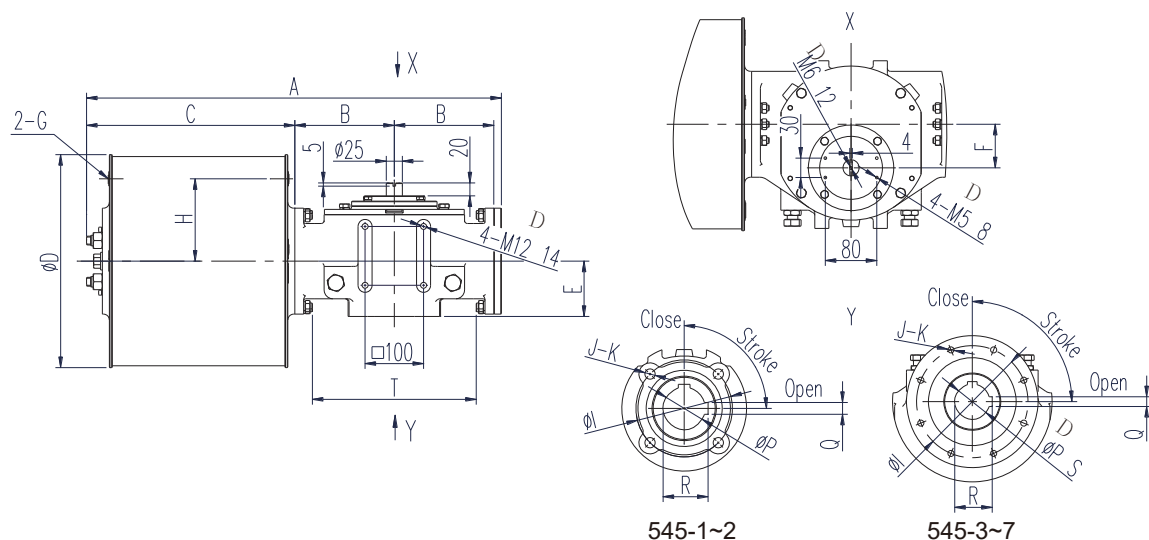
Dimensions - Double acting
