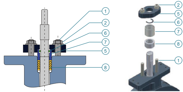
Packing sealing system Standard
