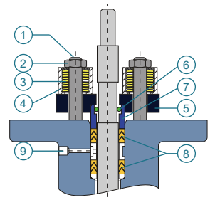
Double-packed live-loaded Monitoring port optional
