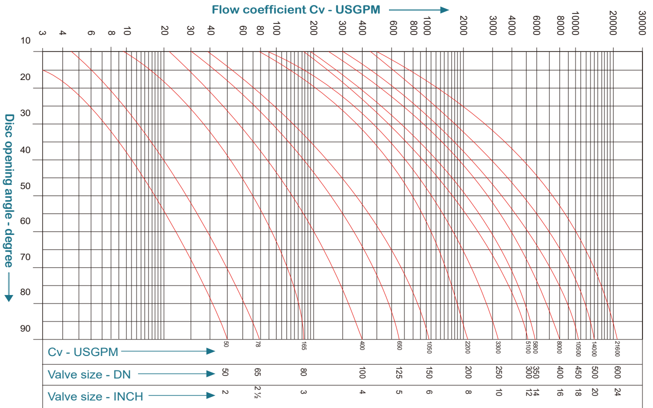
Cv curve - Class150, PN10/16 valves
